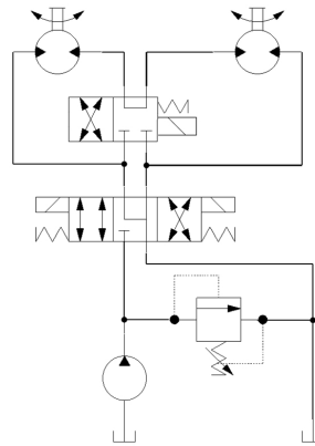
Series/Parallel
